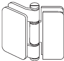
50.0002.-- Glass to glass, overlapping, 180°
