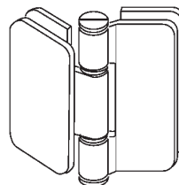
50.0004.135.-- Glass to glass, inward, 135°
