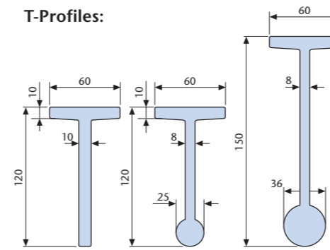
These T-Profiles are typical of the support steelwork.
